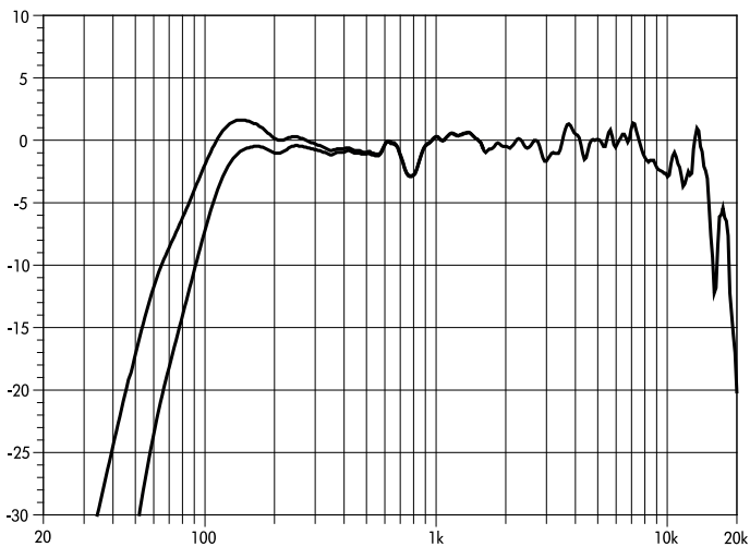
MAX2 frequency response (linear setup, free field), standard and CUT
