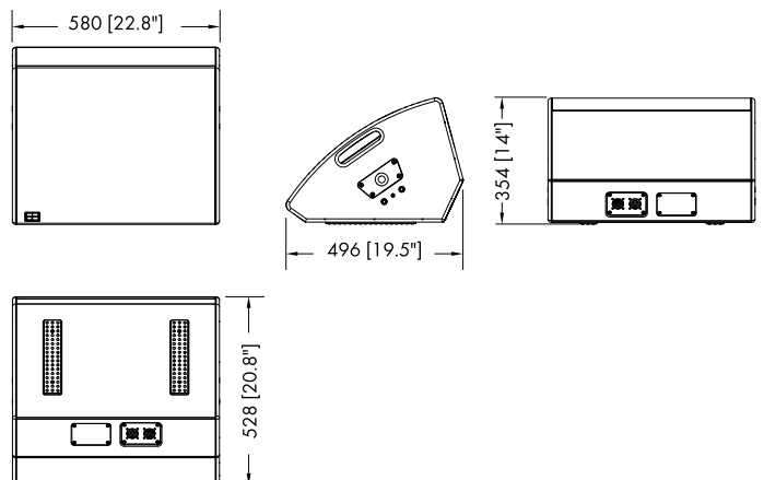
MAX2 cabinet dimensions in mm [inch]
